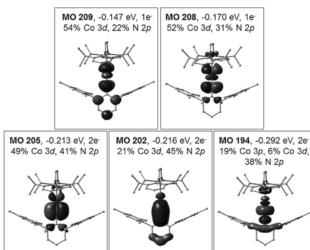
Figure 2. Molecular orbital (MO) plots involving π- and σ-type Co–N interactions for [(IPr)Co(NDmp)] at the S = 3/2 state.
